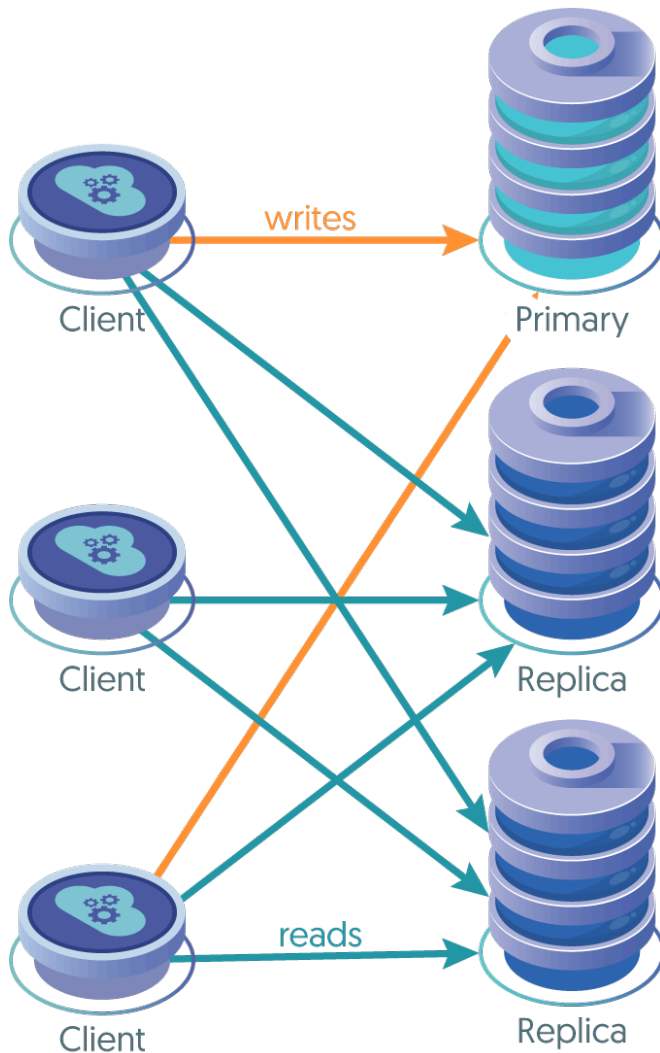
Figure 7.3. Advanced MySQL/Application Connectivity
