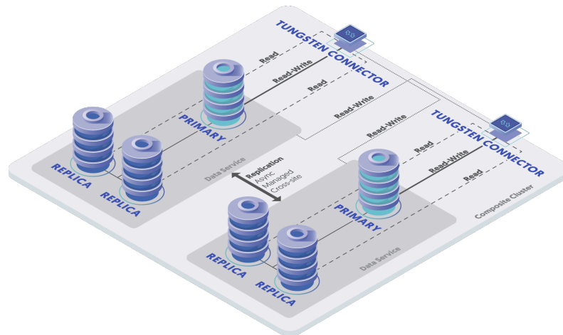
Figure 3.3. Topologies: Composite Active/Active Clusters
