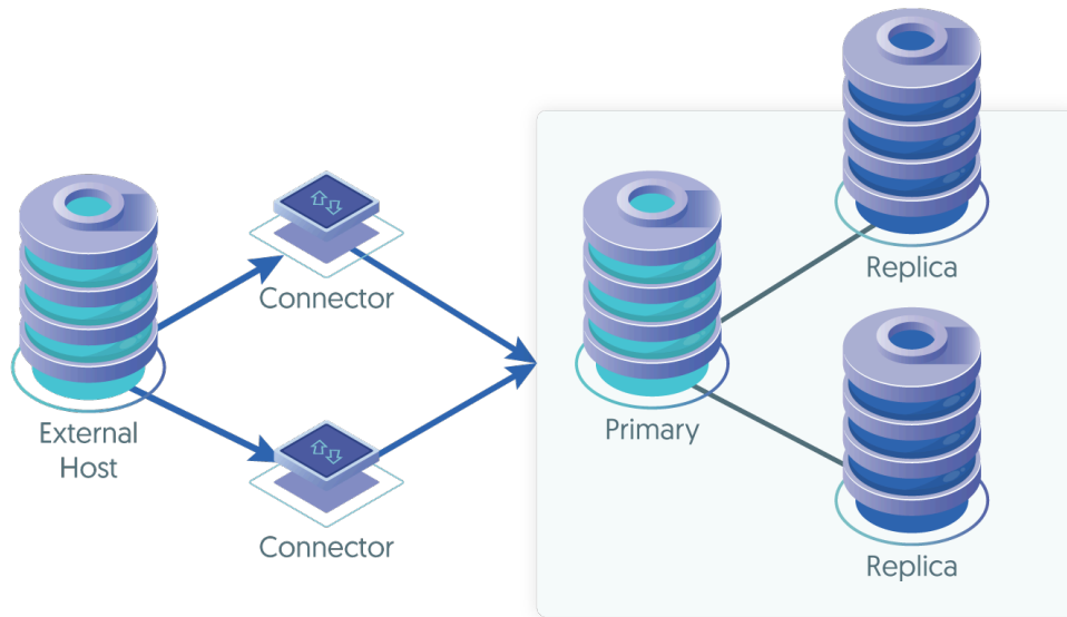
Figure 3.6. Topologies: Replicating into a Dataservice
