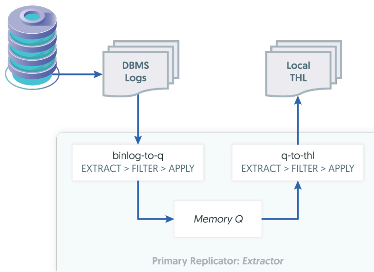
Figure 12.1. Filters: Pipeline Stages on Extractors
