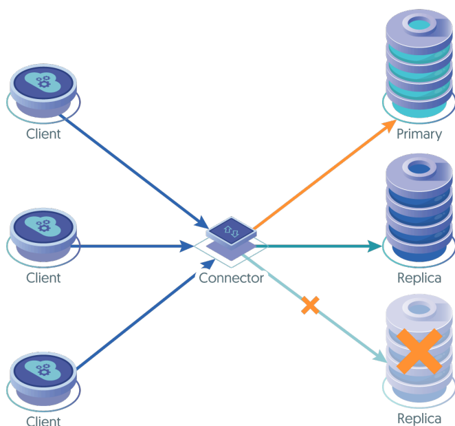
Figure 7.5. Tungsten Connector during a failed datasource
