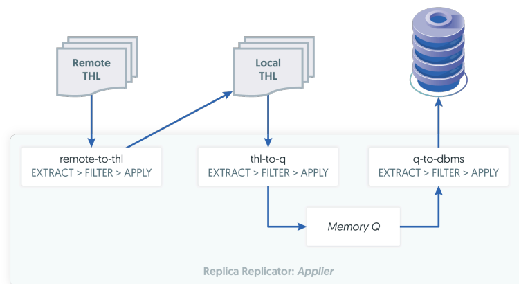
Figure 12.2. Filters: Pipeline Stages on Appliers
