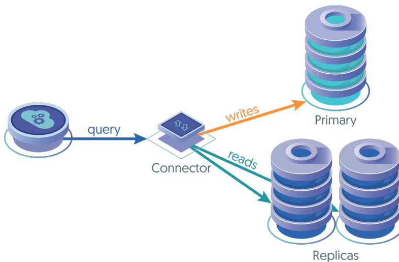
Figure 7.6. Tungsten Connector routing architecture
