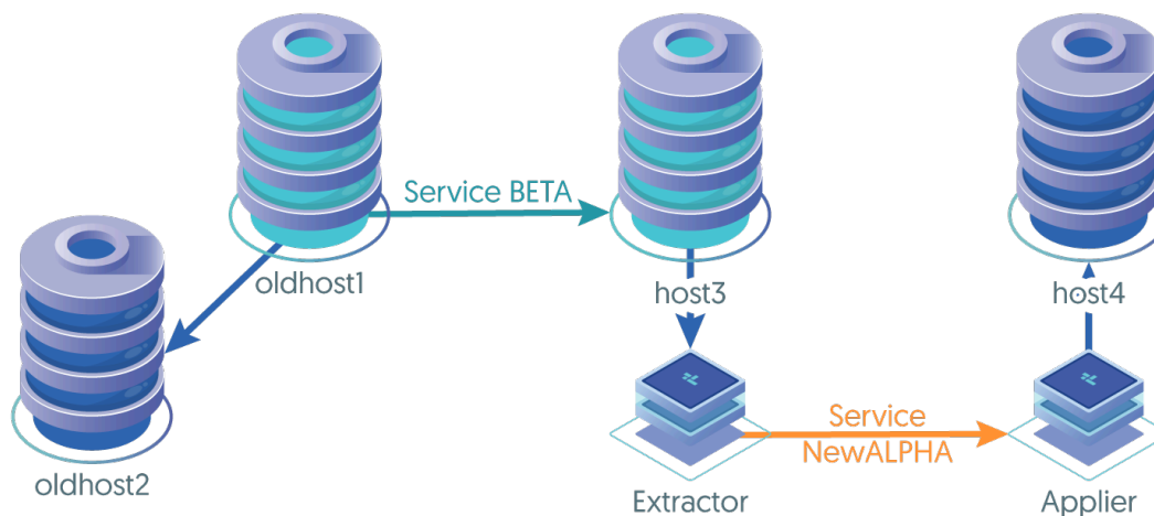
Figure 6.1. Migration: Migrating Native Replication using a New Service
