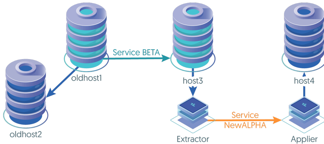
Figure 3.8. Migration: Migrating Native Replication using a New Service
