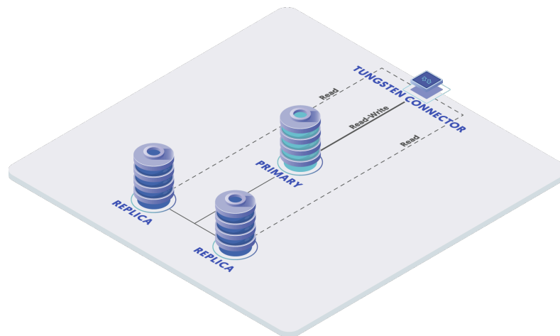
Figure 3.1. Topologies: Standalone HA Cluster
