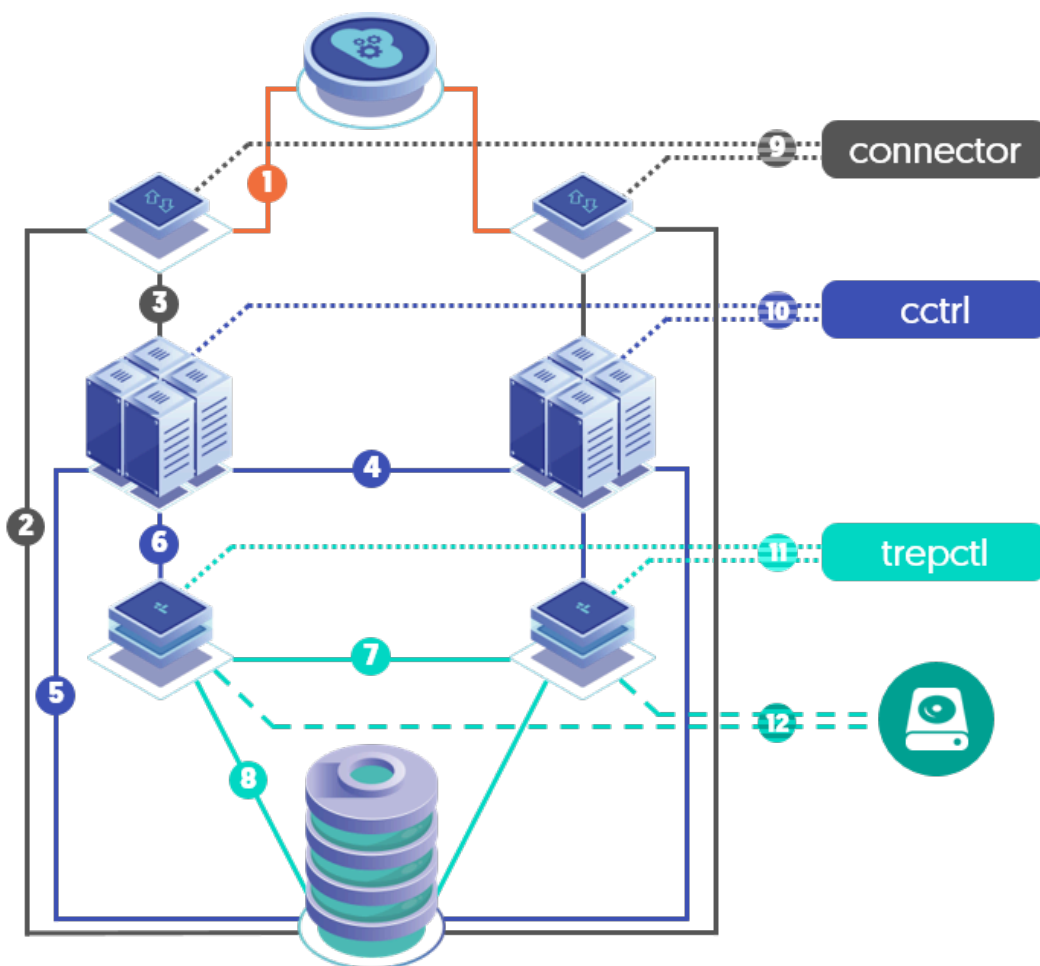
Figure 10.1. Internals: Cluster Communication Channels
