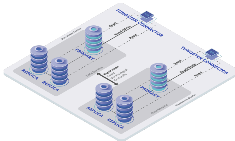
Figure 3.5. Topologies: Multi-Site/Active-Active Clusters
