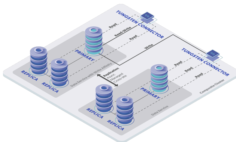
Figure 3.4. Topologies: Composite Dynamic Active/Active Clusters
