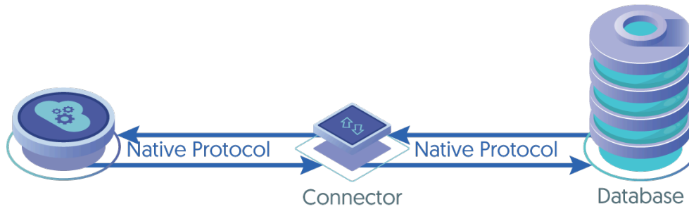
Figure 7.7. Tungsten Connector Bridge Mode Architecture
