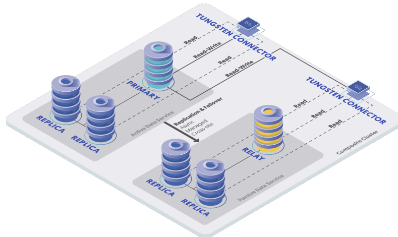
Figure 3.2. Topologies: Composite Active/Passive Cluster
