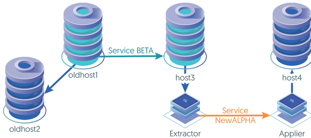
Figure 3.7. Migration: Migrating Native Replication using a New Service
